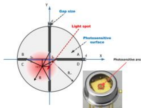
Figure 5: QPD schematic showing spot position v
