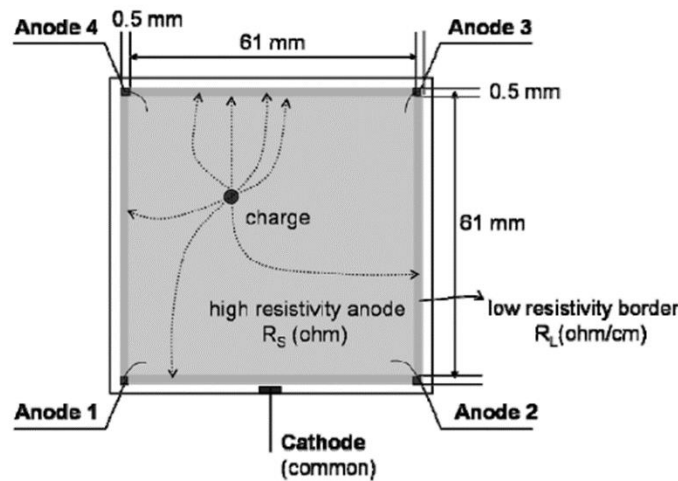
Figure 8: Silicon tetralateral continuous position sensing viii
